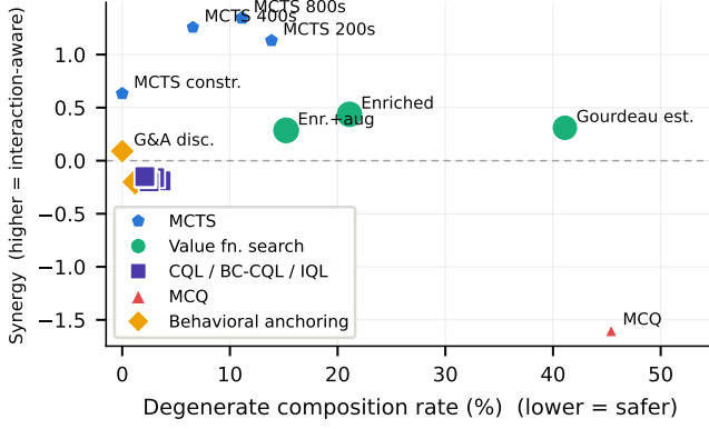
Fig. 2. Safety vs. interaction-awareness (Table IV; MCTS 200s/400s/800s are the leak-free configurations of Table V, searched at inference with root temperature 1, while constrained MCTS is the policy argmax of Table IV; anchored points are the submission’s rich-evaluation runs). Marker size encodes hero diversity. Only MCTS reaches both low degenerate rate and positive synergy; masking pins the degenerate rate at zero.
